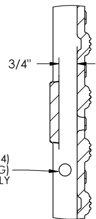
DETAIL C
